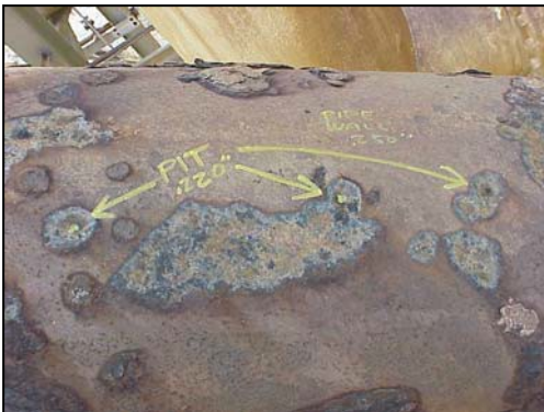
Fig. 2 – Surface preparation as shown is generally unacceptable. In cases where the pipe cannot be properly cleaned, it should be noted that the final ultimate properties of the composite layup may be compromised (such as bonding to the steel surface).
